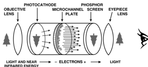
Fig. 1 Image intensification process
